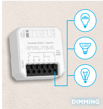
7b RFDEL-71B-SL phase dimmer available for R-L-C-LED loads.
