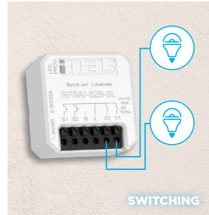
7c The RFSAI-61B-SL (1x8A output) or RFSAI-62B-SL (2x8A outputs) can be used for switching. If you need to switch higher loads, then we offer the RFSAI-61B, which features 16A.
